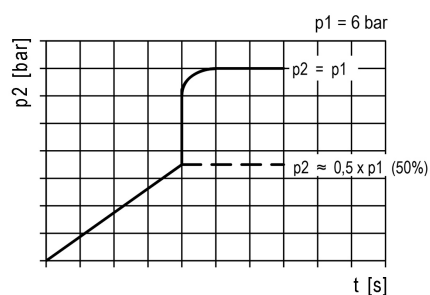
filling characteristic
