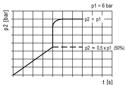
filling characteristic
