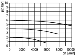
flow characteristic
