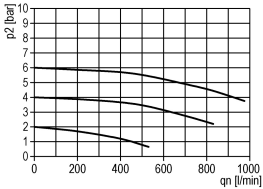
flow characteristic
