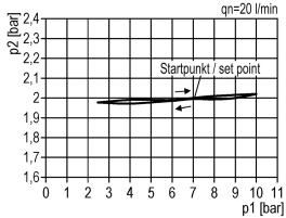
pressure characteristic
